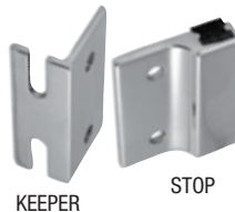
KEEPER BUMPER For Outswing 1-1/2" bet. screws Flat surface type Part No. 9A5260 Chrome Part No. 9A5263 Cast SS
